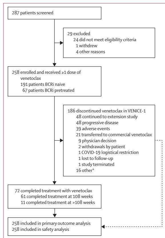
Figure 1: Study profile
